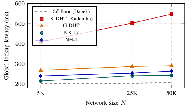
Fig. 4. Global-lookup latency vs network size, plotted against the Dabek 3\delta analytical floor (gray dashed). NX-17 plateaus at 1.18\times the floor at 25 000 and 50 000 nodes; NH-1 at 1.28\times . Kademlia worsens from 2.01\times to 2.65\times over the same range. The floor itself is essentially flat ( \delta is a property of the network, not of N ).
