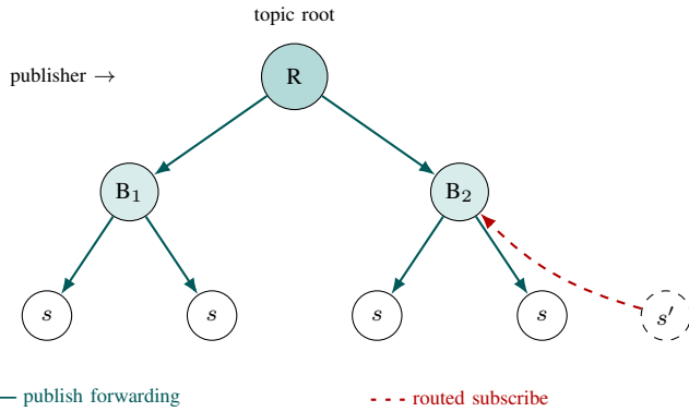
Fig. 3. Axon-tree formation. A new subscriber s' issues a routed SUBSCRIBE toward topicId (red dashed); the first live axon role on the path (here, B_2 ) intercepts and adopts it. Publishes flow from the root R through the branches to all subscribers (teal solid). Tree healing under churn is the same mechanism: a subscriber whose parent dies re-issues its subscribe, attaches to whichever live ancestor is now closest, and continues receiving publishes after one refresh interval.
